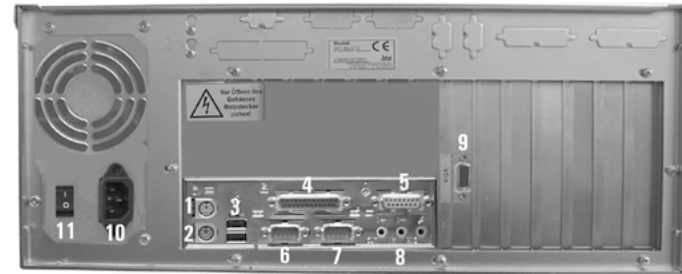
Picture: connection panel IPC-B with ITX/ATX-Board (Example, depending on used mother- board)
