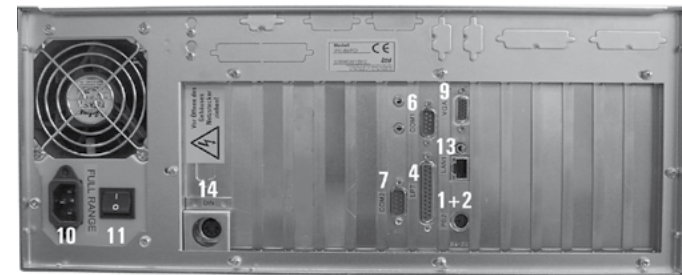
Picture: connection panel IPC-B with backplane (Example, depending on used hardware and components)
