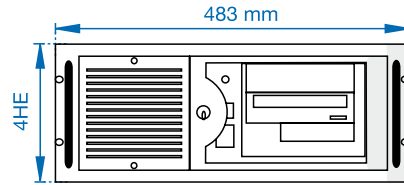
Frontansicht Front view
