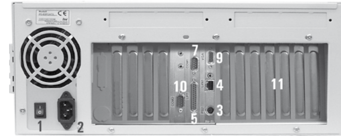
Picture: connection panel IPC-ECO with backplane (Example, depending on used hardware and components)
