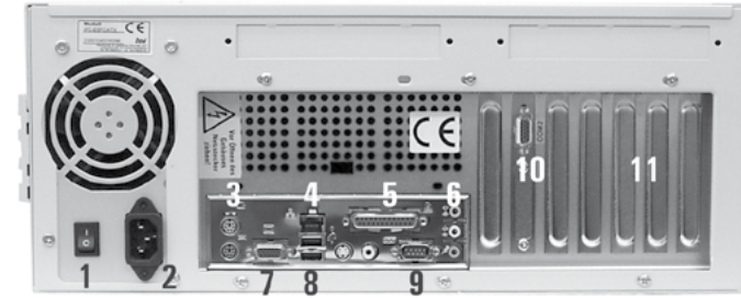
Picture: connection panel IPC-ECO with ITX/ATX-Board (Example, depending on used motherboard)
